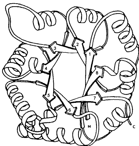
Figure 2. Parallel (\beta/\alpha)_8 -barrel of triosephosphate isomerase This structure illustrates the classical TIM-barrel fold and is used as an illustrative example. The motif is composed of eight parallel \beta -strands (numbers 1–8) forming the inner \beta -barrel sheet that is surrounded by eight \alpha -helices in such a way that there are eight repeated (\beta\alpha) -units in a regular (\alpha/\beta)_8 -barrel. The motif is seen in the end view, i.e. the C-terminal end of the \beta -barrel is toward the reader. Adapted from Richardson (1981)
