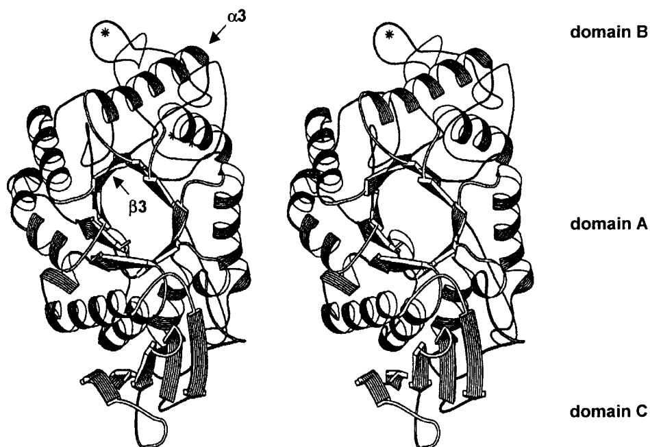
Figure 3. Overall structure of barley \alpha -amylase in stereo. The structure consists of three domains: A, a parallel (\beta/\alpha)_8 -barrel, B, an irregular fold stabilised by three calcium ions (stars); and C, a 5-stranded anti-parallel \beta -sheet. The third \beta -strand ( \beta 3 ) and third \alpha -helix ( \alpha 3 ) are also marked. Adapted from Kadziola et al. (1994)
